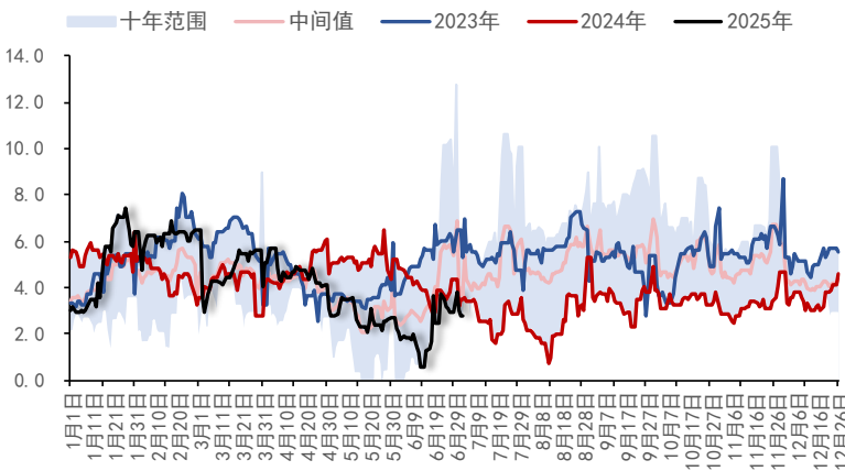
图33: MRBN/WTI ($/桶)
