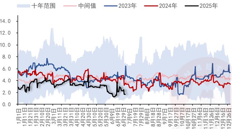
图30: Brent/WTI ($/桶)
