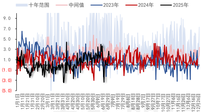
图31: Brent/Dubai ($/桶)
